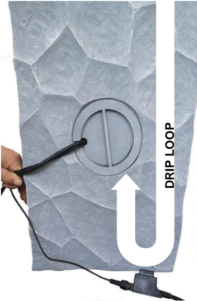
To prevent the risk of water loss, create a drip-loop with the light cord inside the fountain.
